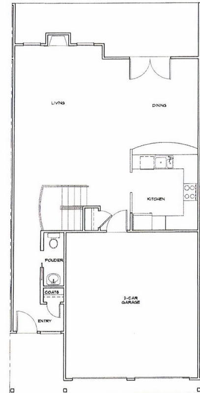
1 CL FIRST FLOOR PLAN
