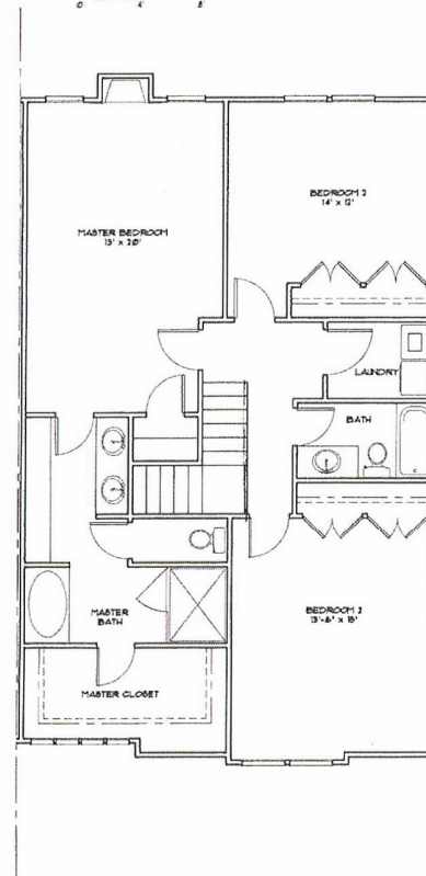
2 CL SECOND FLOOR PLAN
